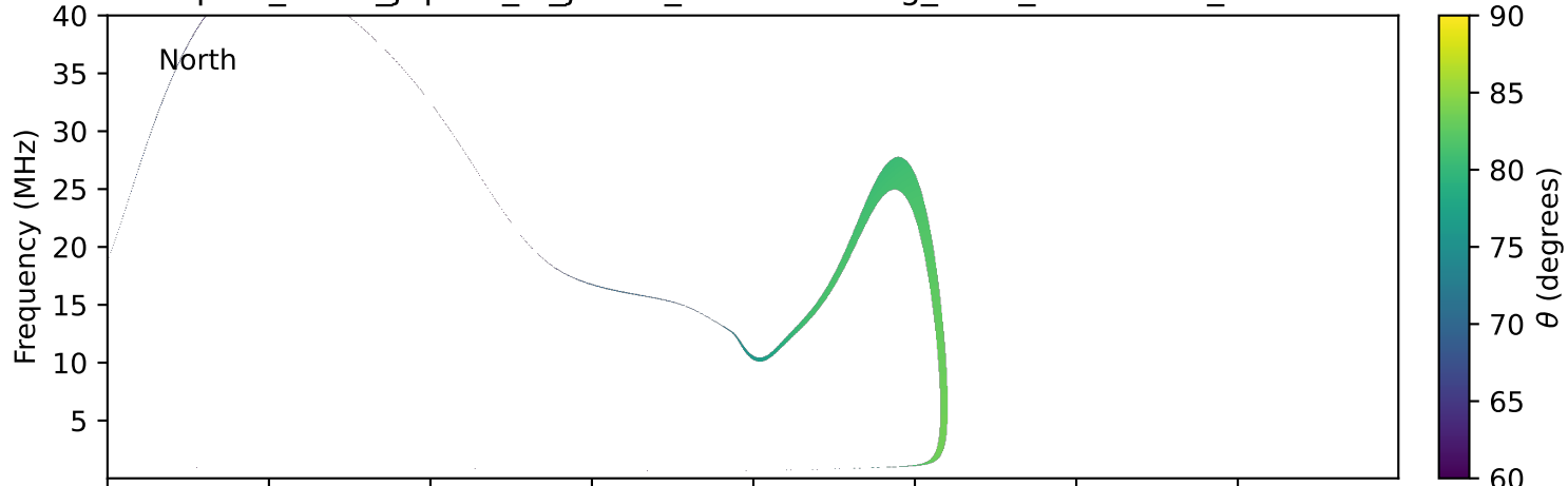
expres_earth_jupiter_io_jrm09_lossc-wid1deg_3kev_19910108_v11.cdf
