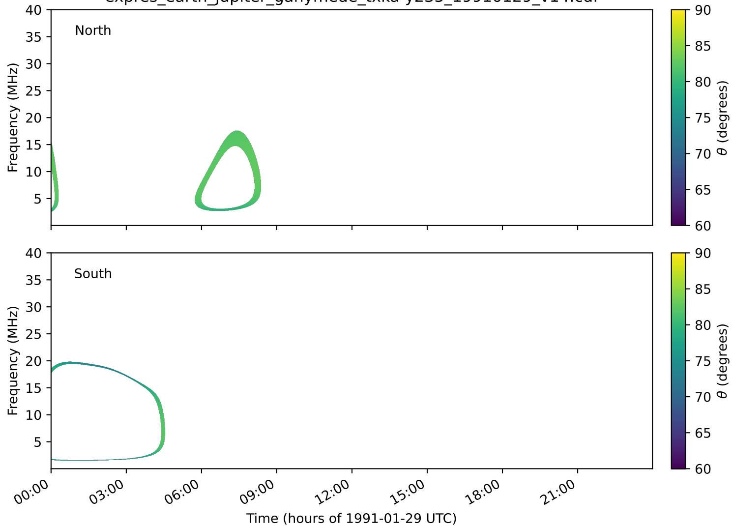
expres_earth_jupiter_ganymede_txka-y235_19910129_v14.cdf
