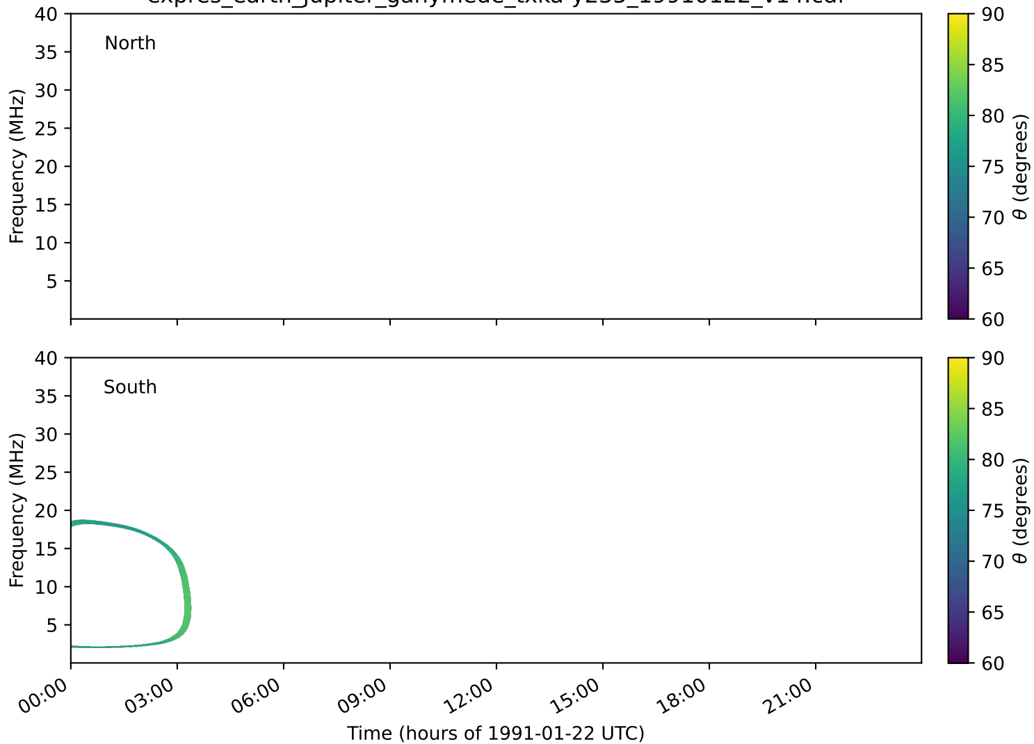
expres_earth_jupiter_ganymede_txka-y235_19910122_v14.cdf
