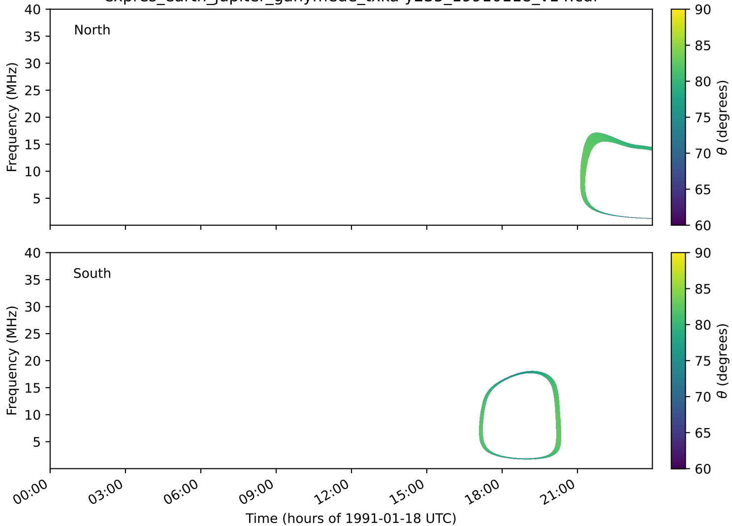
expres_earth_jupiter_ganymede_txka-y235_19910118_v14.cdf
