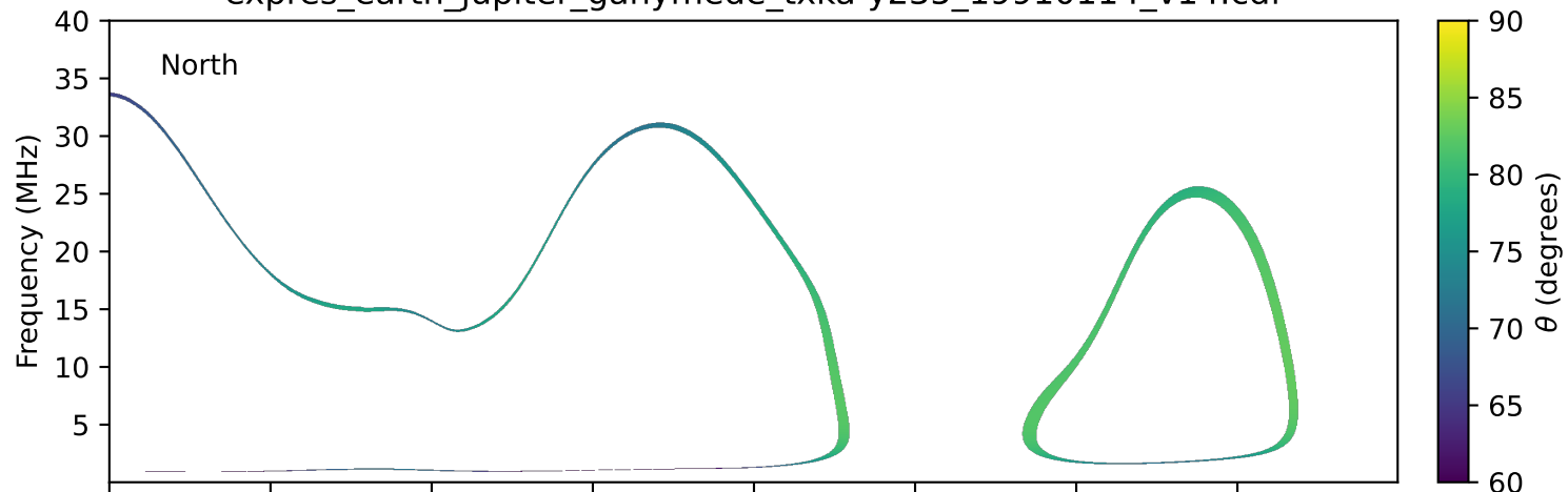
expres_earth_jupiter_ganymede_txka-y235_19910114_v14.cdf
