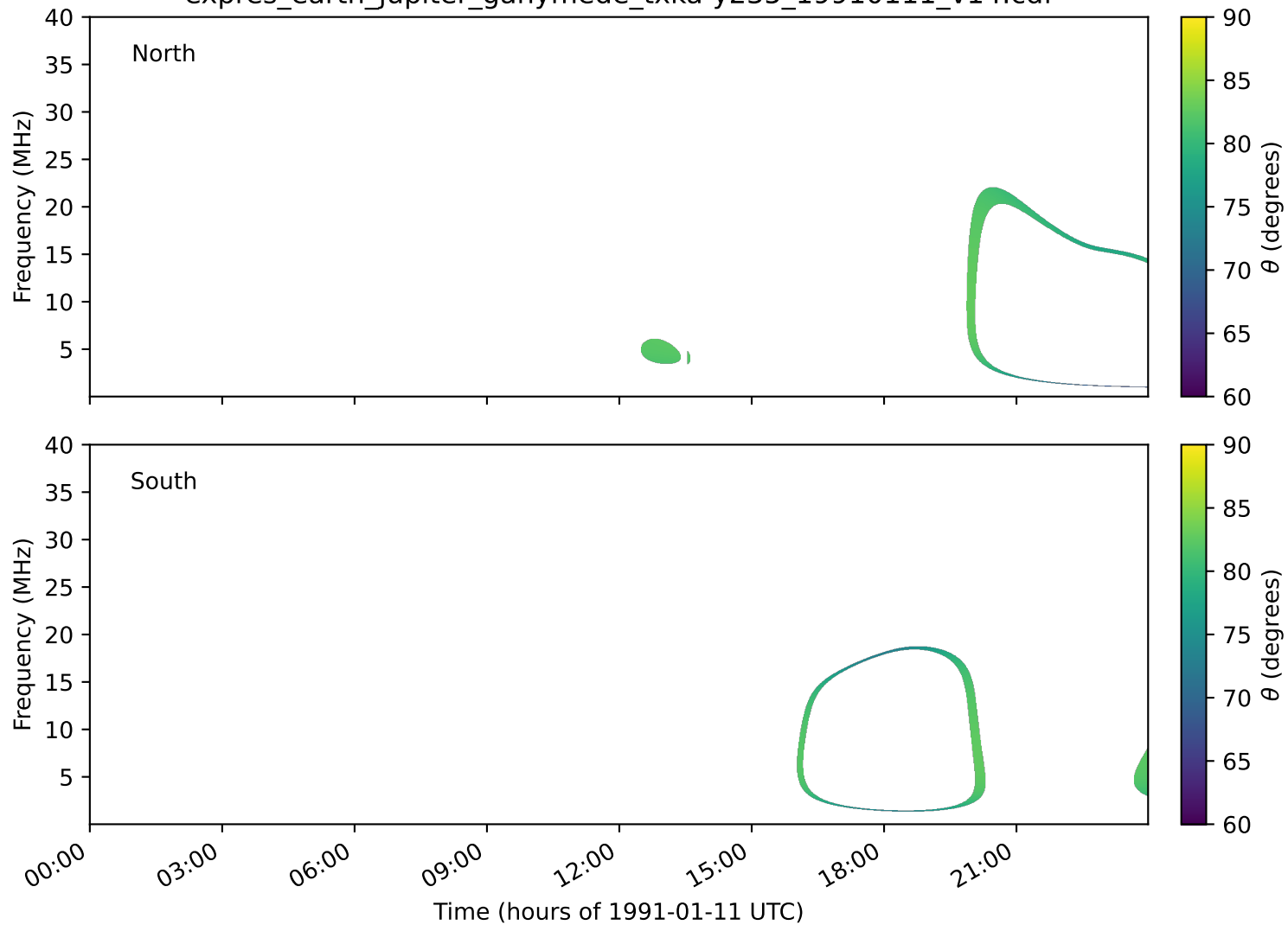
expres_earth_jupiter_ganymede_txka-y235_19910111_v14.cdf
