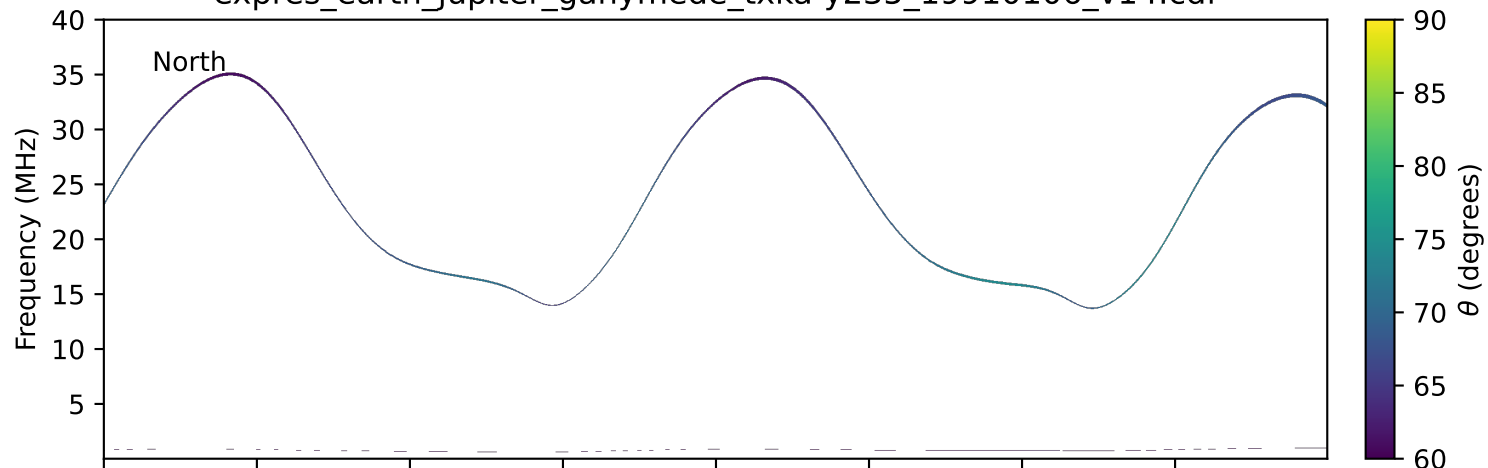
expres_earth_jupiter_ganymede_txka-y235_19910106_v14.cdf
