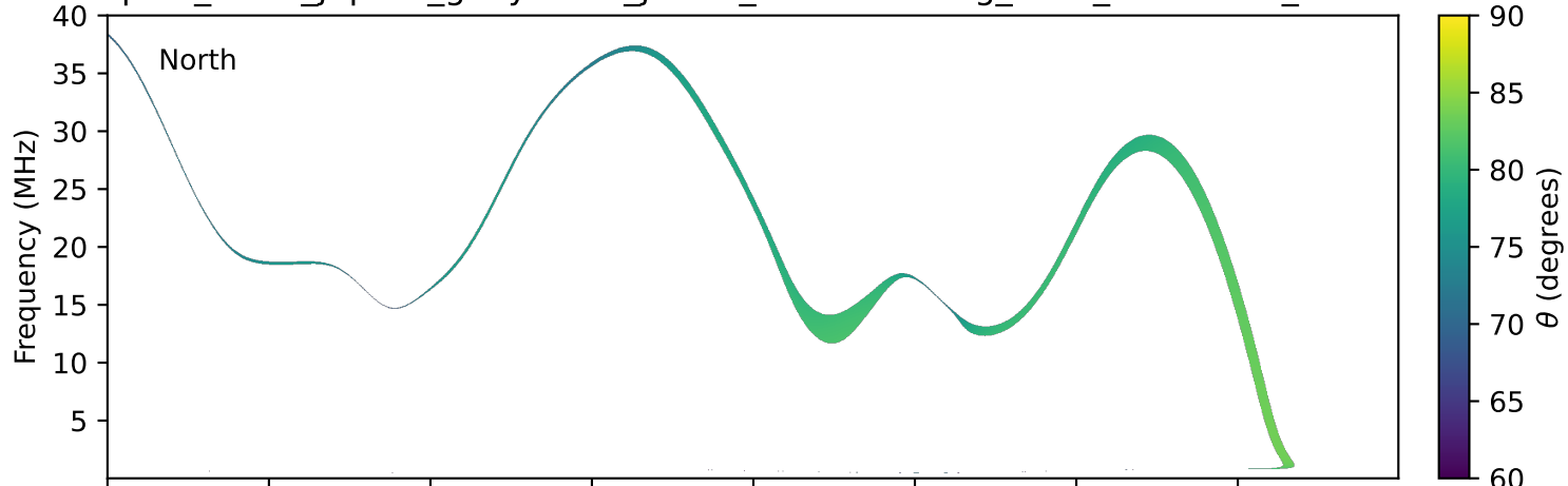
expres_earth_jupiter_ganymede_jrm33_lossc-wid1deg_3kev_19910107_v11.cdf
