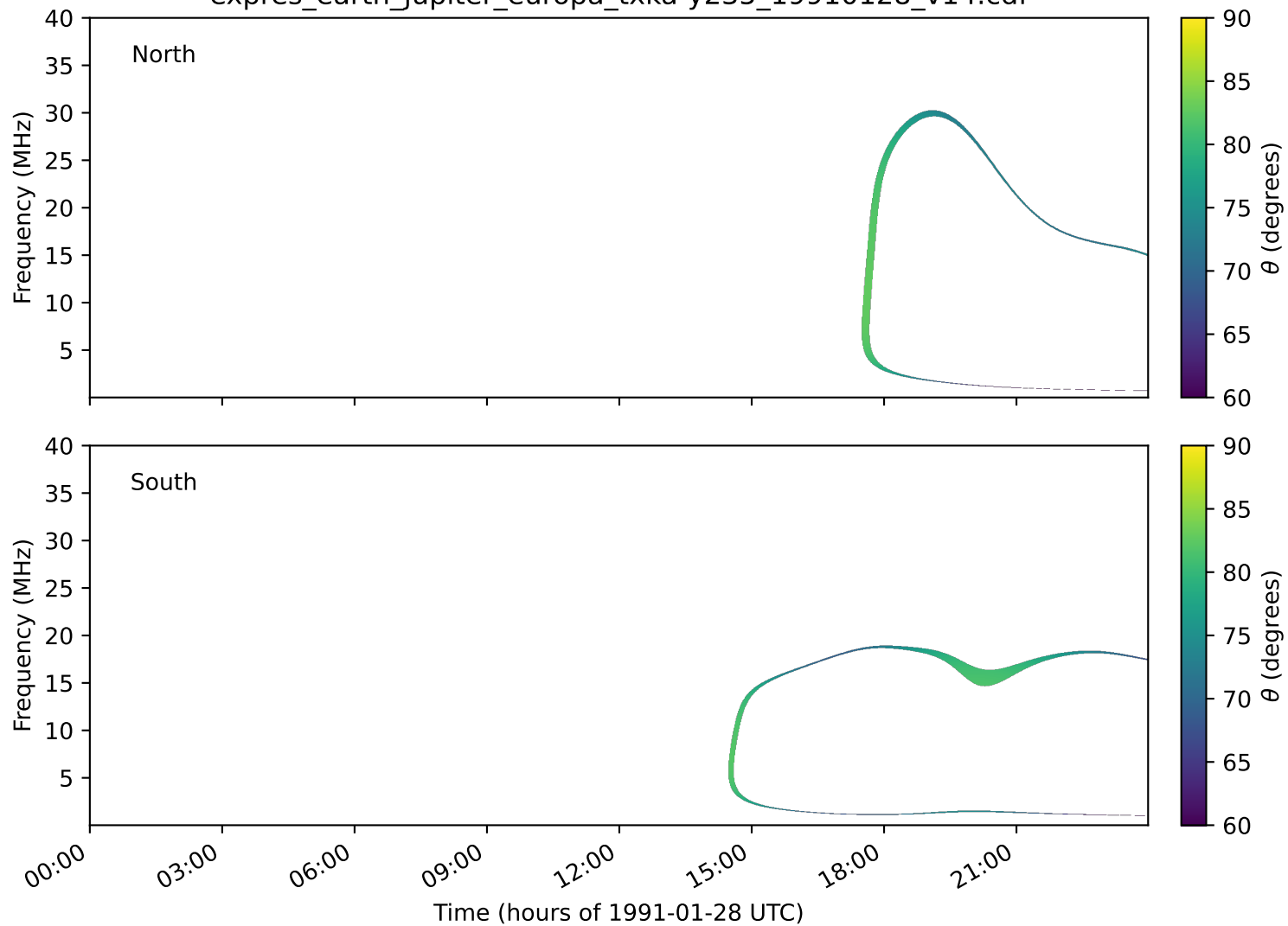
expres_earth_jupiter_europa_txka-y235_19910128_v14.cdf
