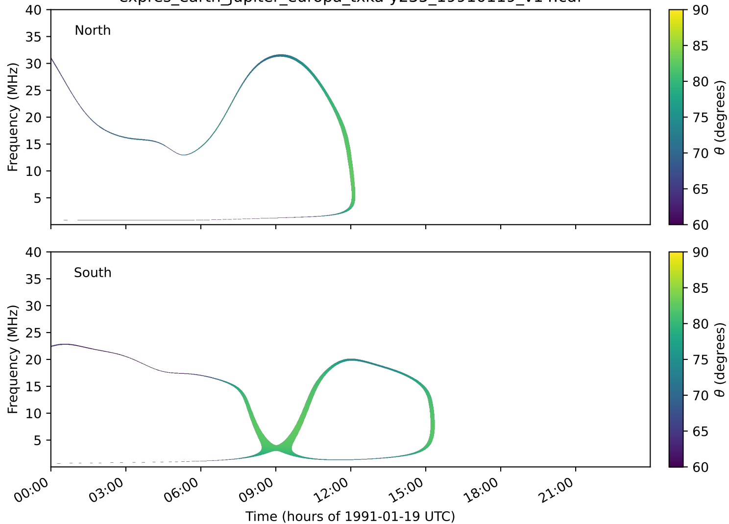
expres_earth_jupiter_europa_txka-y235_19910119_v14.cdf
