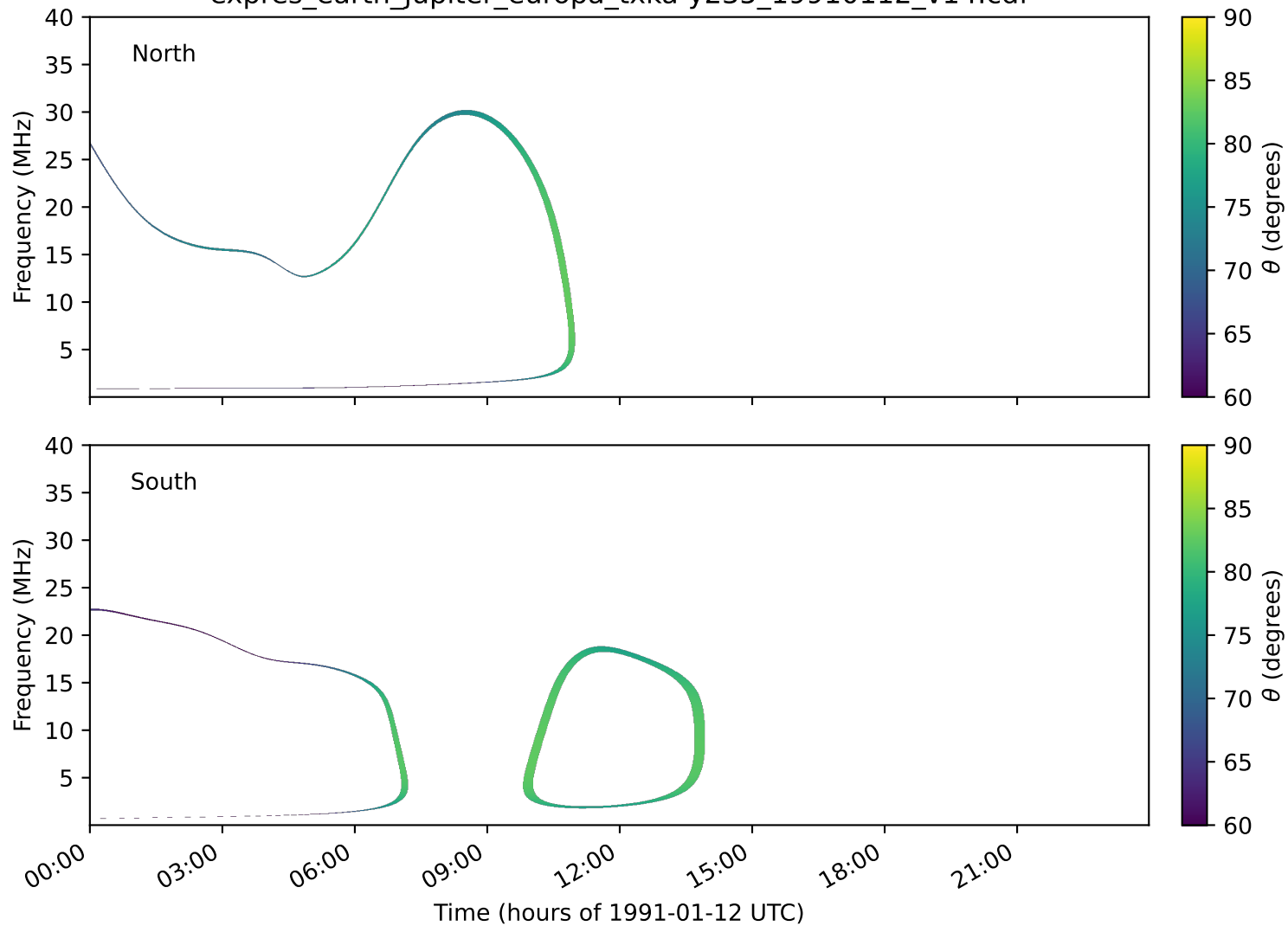
expres_earth_jupiter_europa_txka-y235_19910112_v14.cdf
