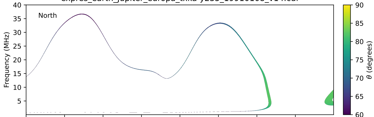
expres_earth_jupiter_europa_txka-y235_19910108_v14.cdf
