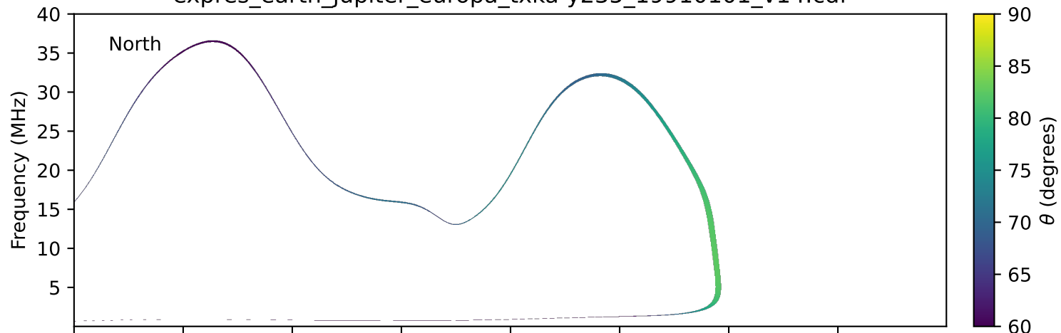
expres_earth_jupiter_europa_txka-y235_19910101_v14.cdf
