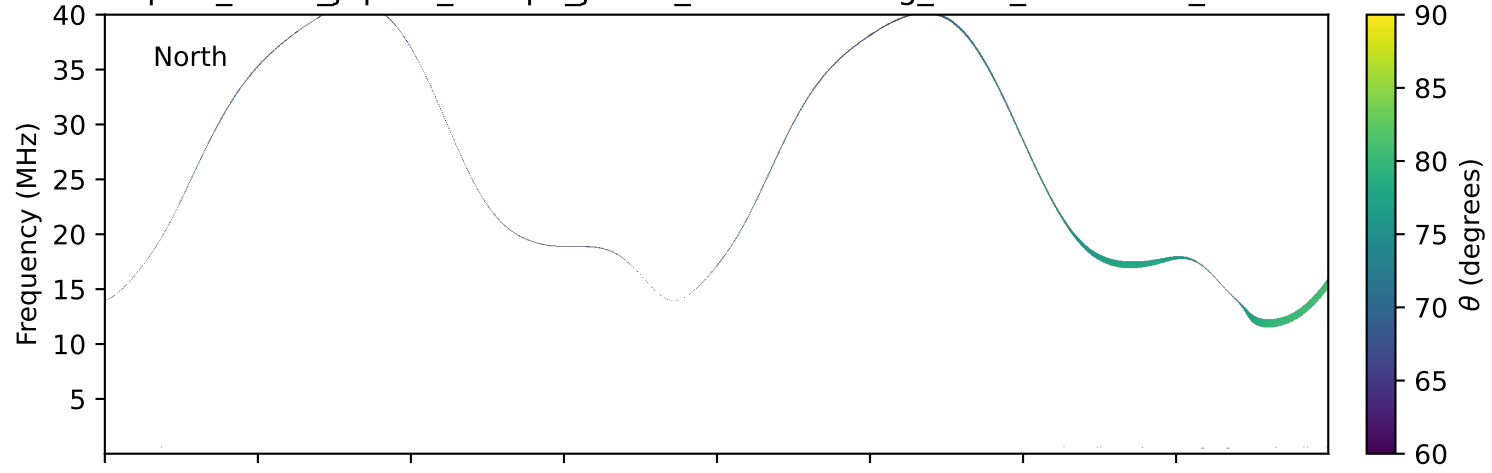
expres_earth_jupiter_europa_jrm33_lossc-wid1deg_3kev_19910115_v11.cdf
