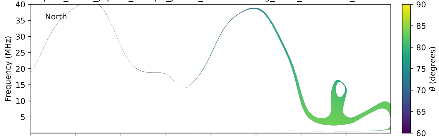
expres_earth_jupiter_europa_jrm33_lossc-wid1deg_3kev_19910101_v11.cdf
