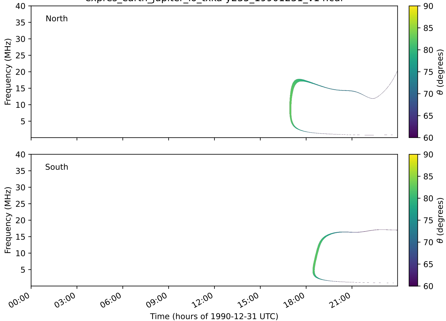
expres_earth_jupiter_io_txka-y235_19901231_v14.cdf
