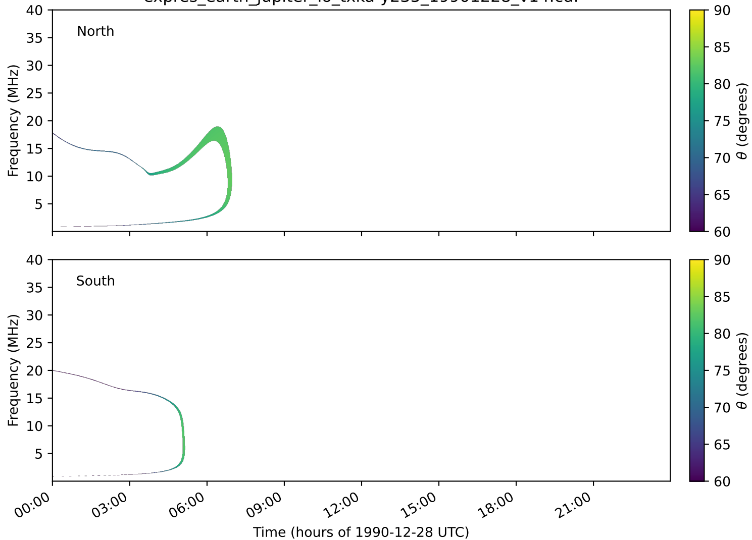
expres_earth_jupiter_io_txka-y235_19901228_v14.cdf
