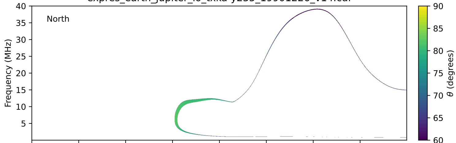
expres_earth_jupiter_io_txka-y235_19901226_v14.cdf
