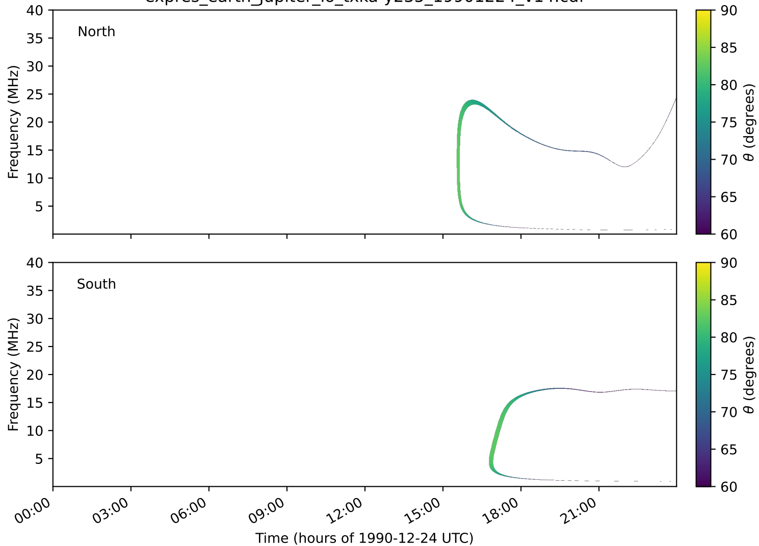
expres_earth_jupiter_io_txka-y235_19901224_v14.cdf
