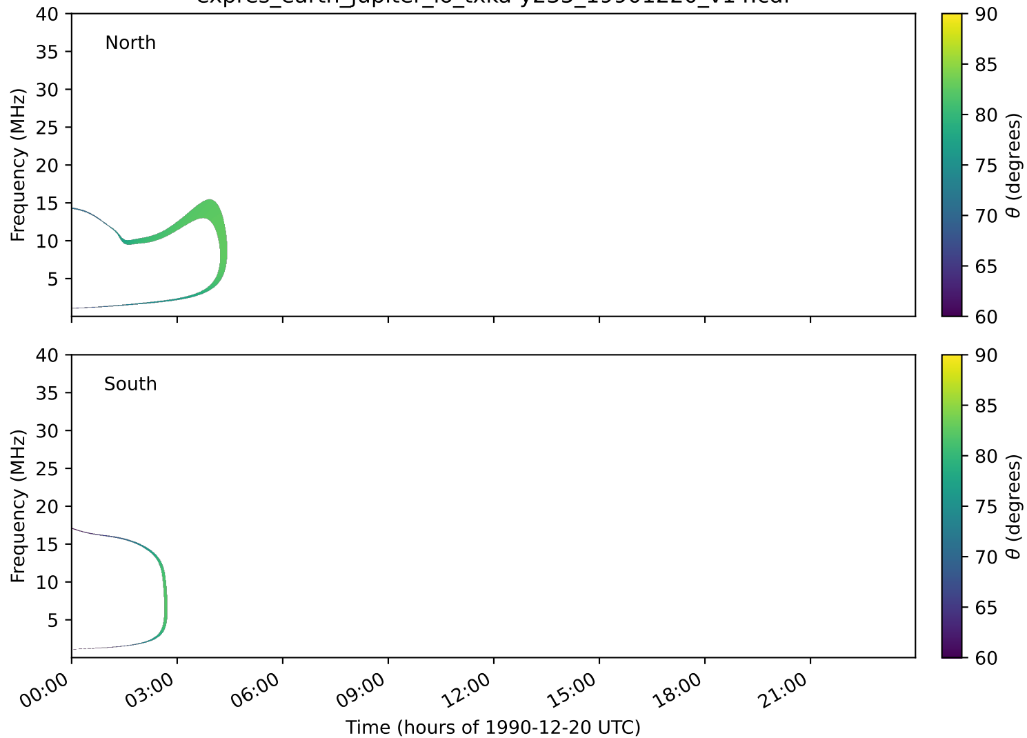
expres_earth_jupiter_io_txka-y235_19901220_v14.cdf
