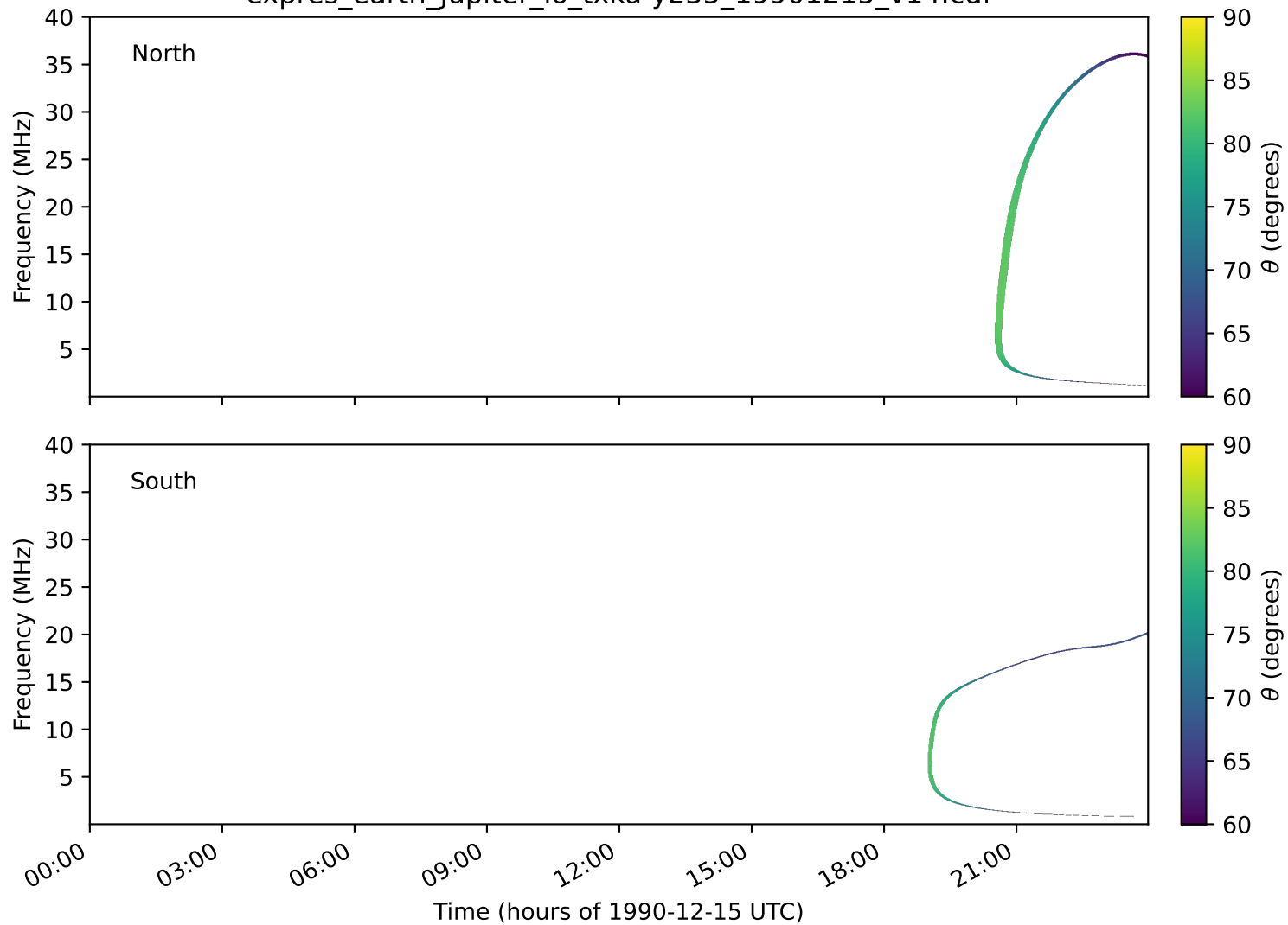
expres_earth_jupiter_io_txka-y235_19901215_v14.cdf
