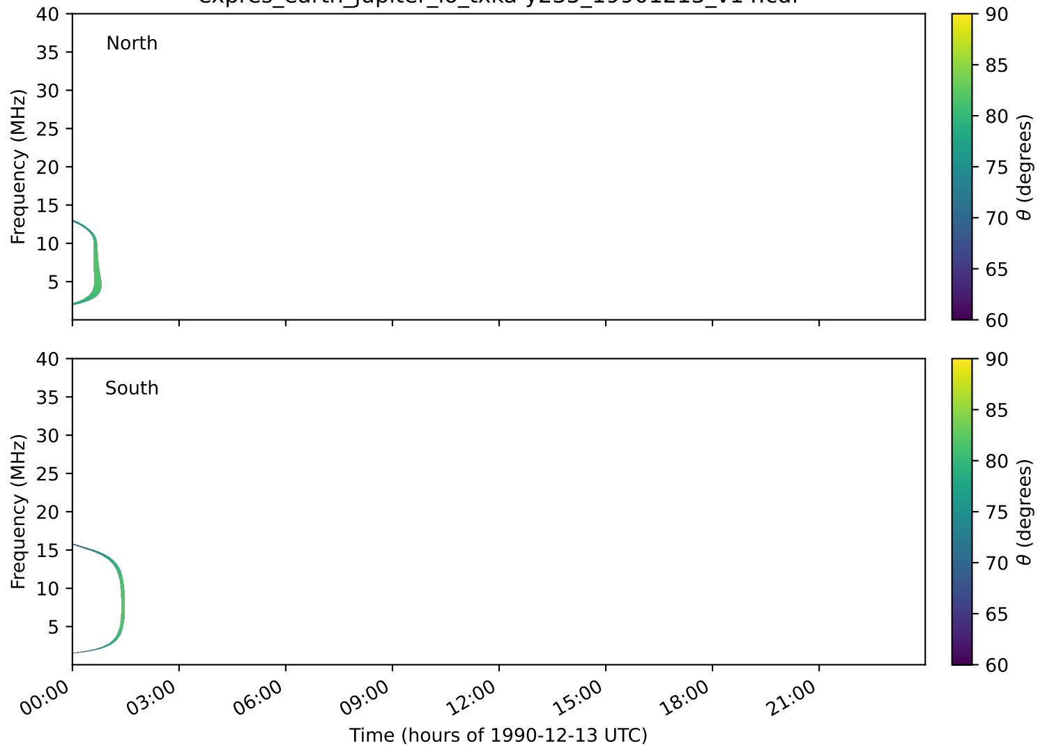
expres_earth_jupiter_io_txka-y235_19901213_v14.cdf
