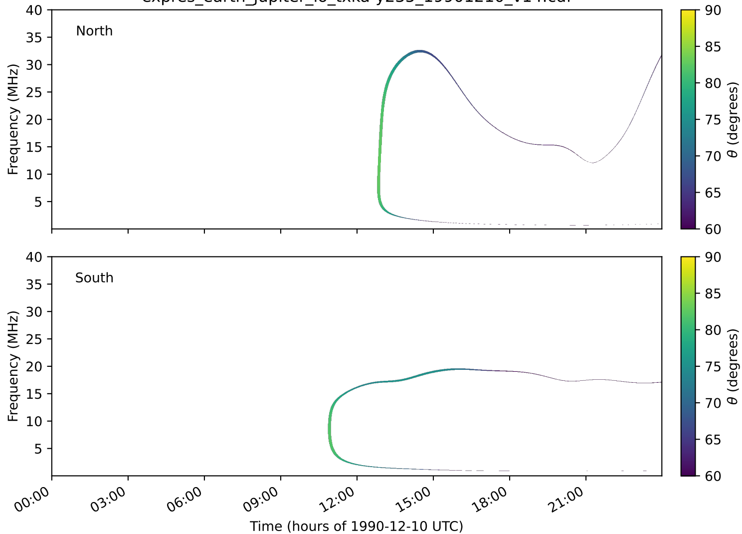
expres_earth_jupiter_io_txka-y235_19901210_v14.cdf
