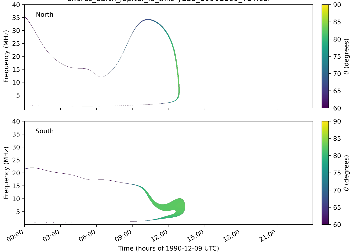
expres_earth_jupiter_io_txka-y235_19901209_v14.cdf
