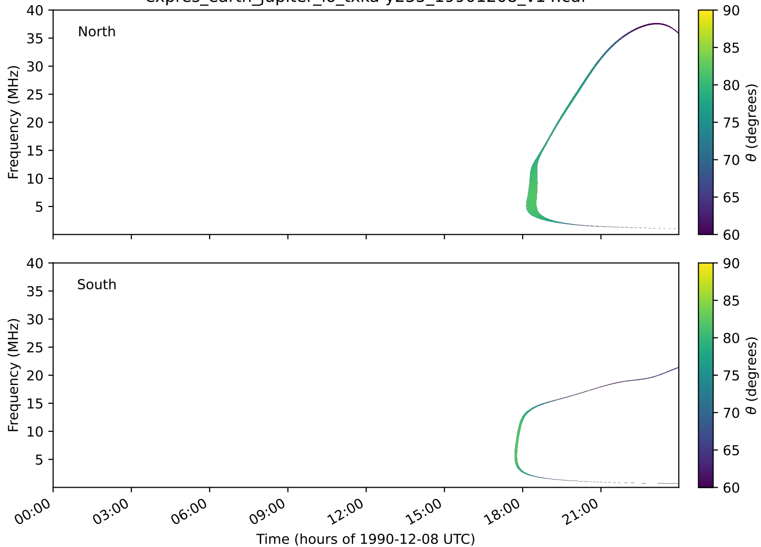
expres_earth_jupiter_io_txka-y235_19901208_v14.cdf
