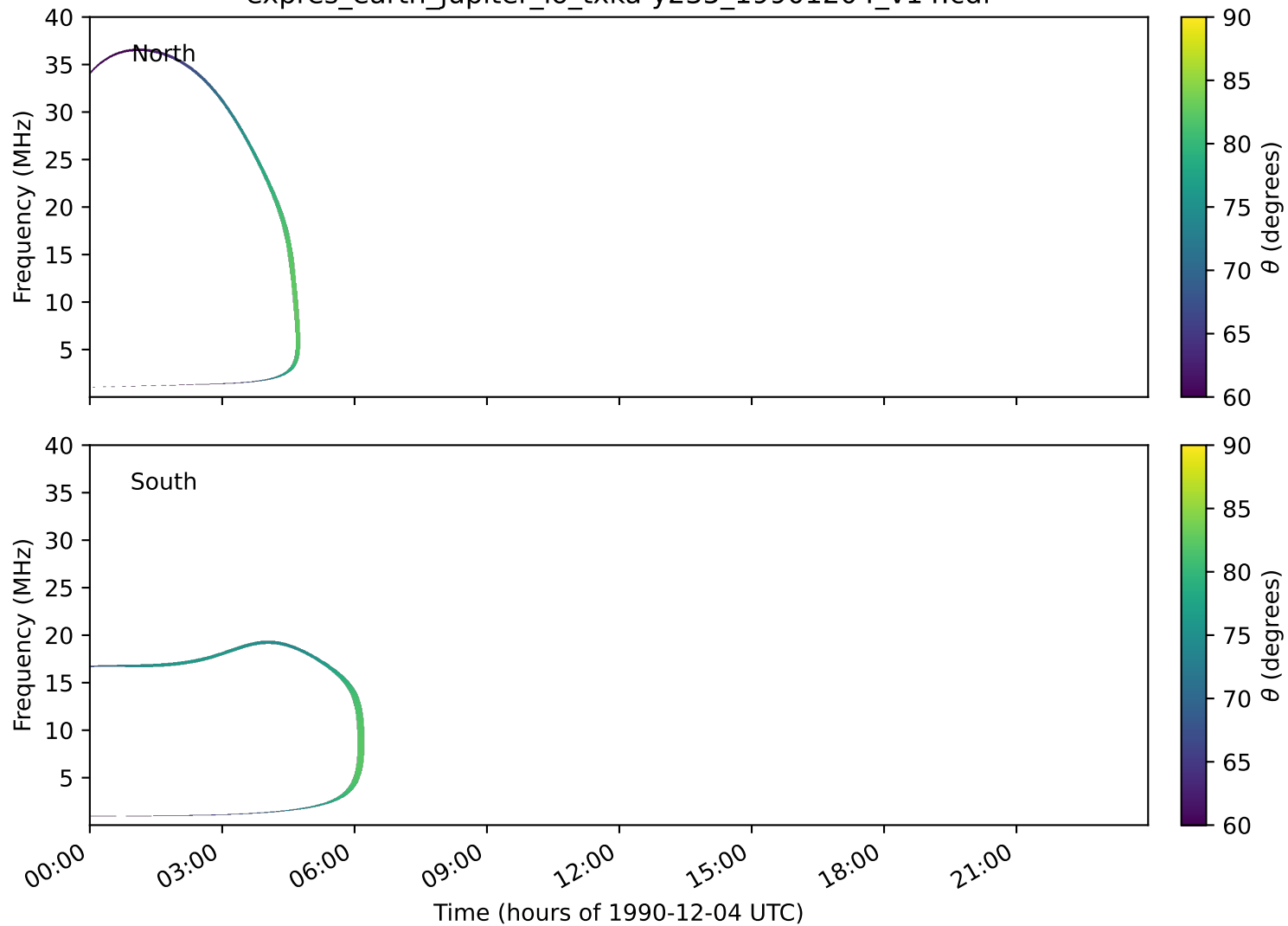
expres_earth_jupiter_io_txka-y235_19901204_v14.cdf
