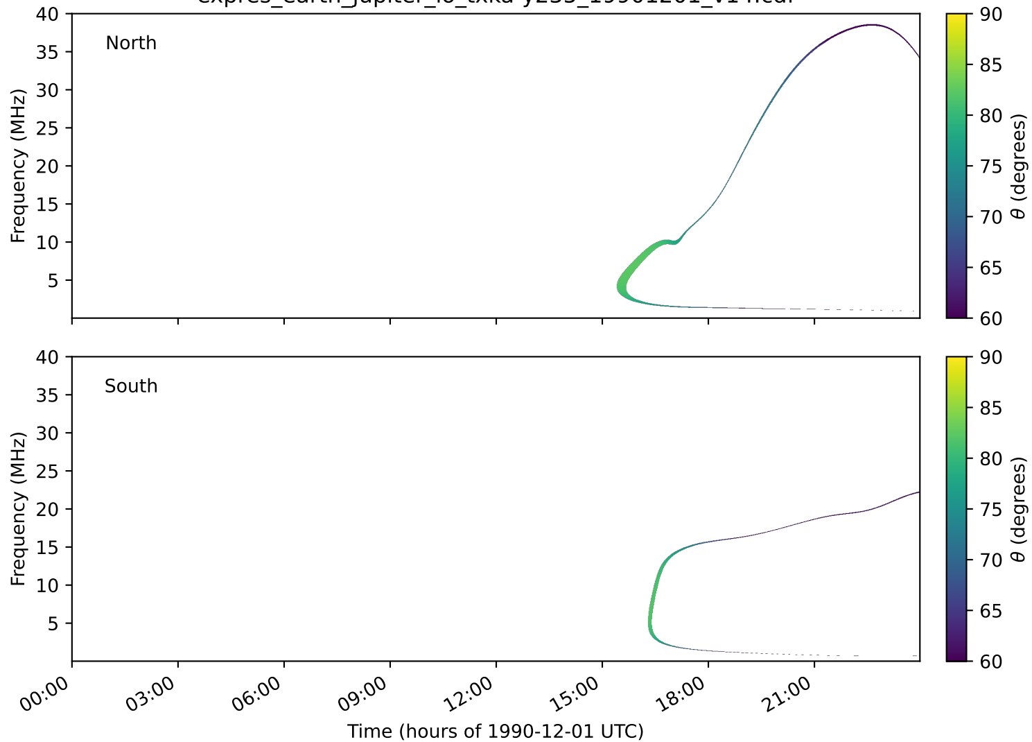
expres_earth_jupiter_io_txka-y235_19901201_v14.cdf
