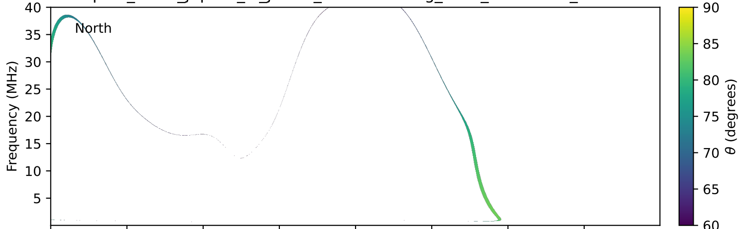
expres_earth_jupiter_io_jrm33_lossc-wid1deg_3kev_19901230_v11.cdf
