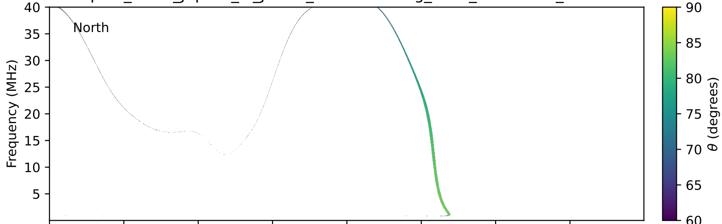
expres_earth_jupiter_io_jrm33_lossc-wid1deg_3kev_19901223_v11.cdf
