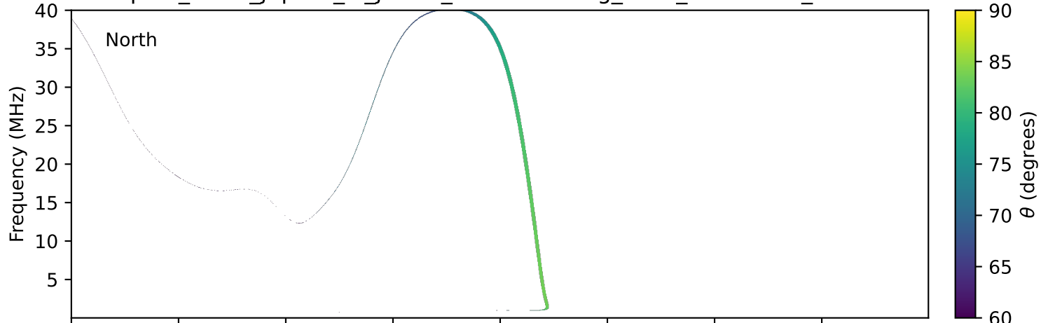
expres_earth_jupiter_io_jrm33_lossc-wid1deg_3kev_19901209_v11.cdf
