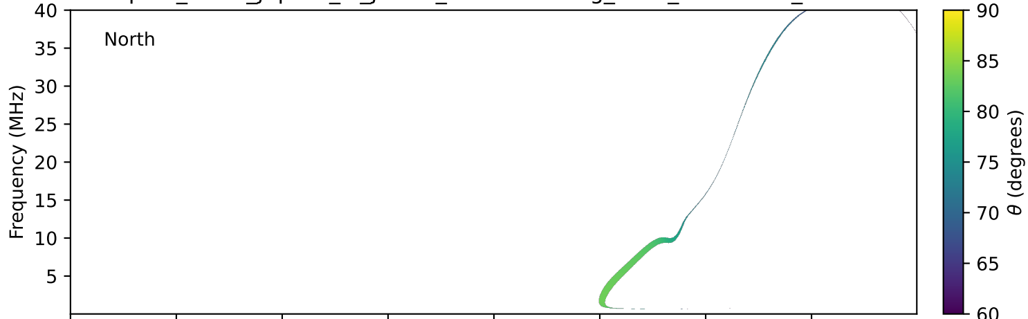
expres_earth_jupiter_io_jrm33_lossc-wid1deg_3kev_19901201_v11.cdf
