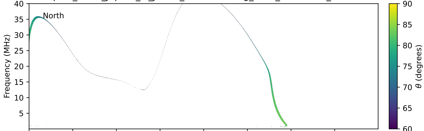
expres_earth_jupiter_io_jrm09_lossc-wid1deg_3kev_19901230_v11.cdf
