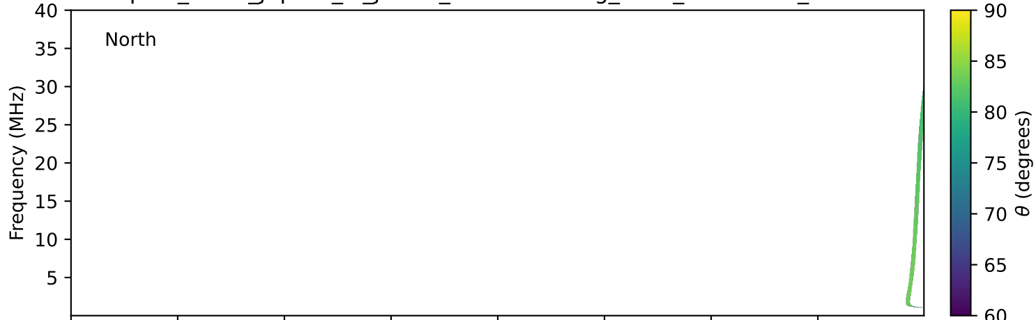
expres_earth_jupiter_io_jrm09_lossc-wid1deg_3kev_19901229_v11.cdf
