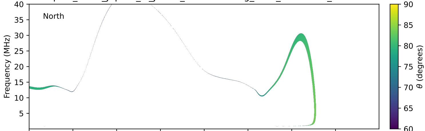
expres_earth_jupiter_io_jrm09_lossc-wid1deg_3kev_19901207_v11.cdf
