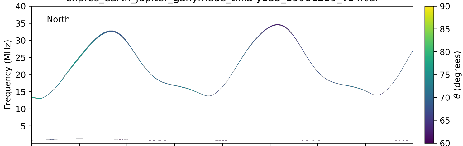
expres_earth_jupiter_ganymede_txka-y235_19901229_v14.cdf
