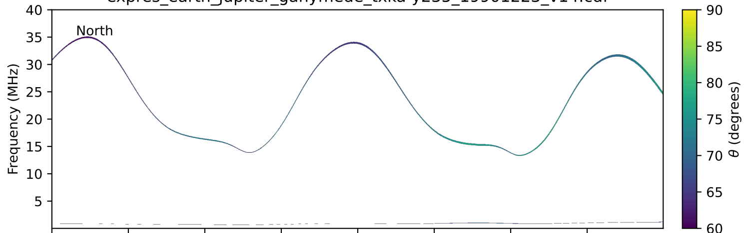
expres_earth_jupiter_ganymede_txka-y235_19901223_v14.cdf
