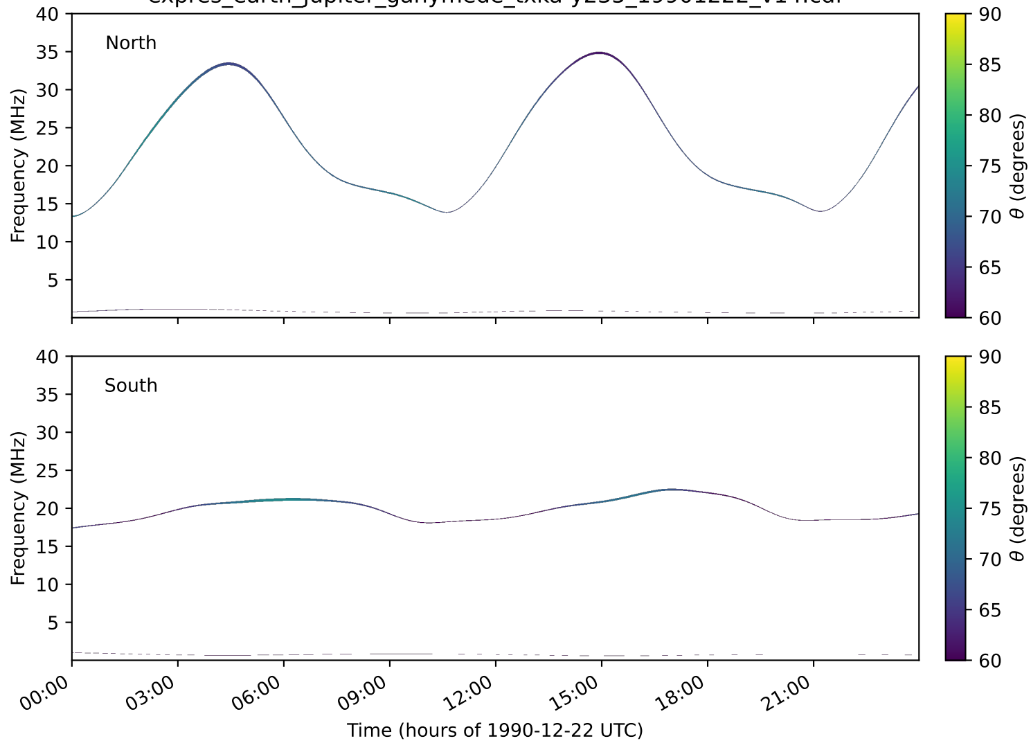
expres_earth_jupiter_ganymede_txka-y235_19901222_v14.cdf
