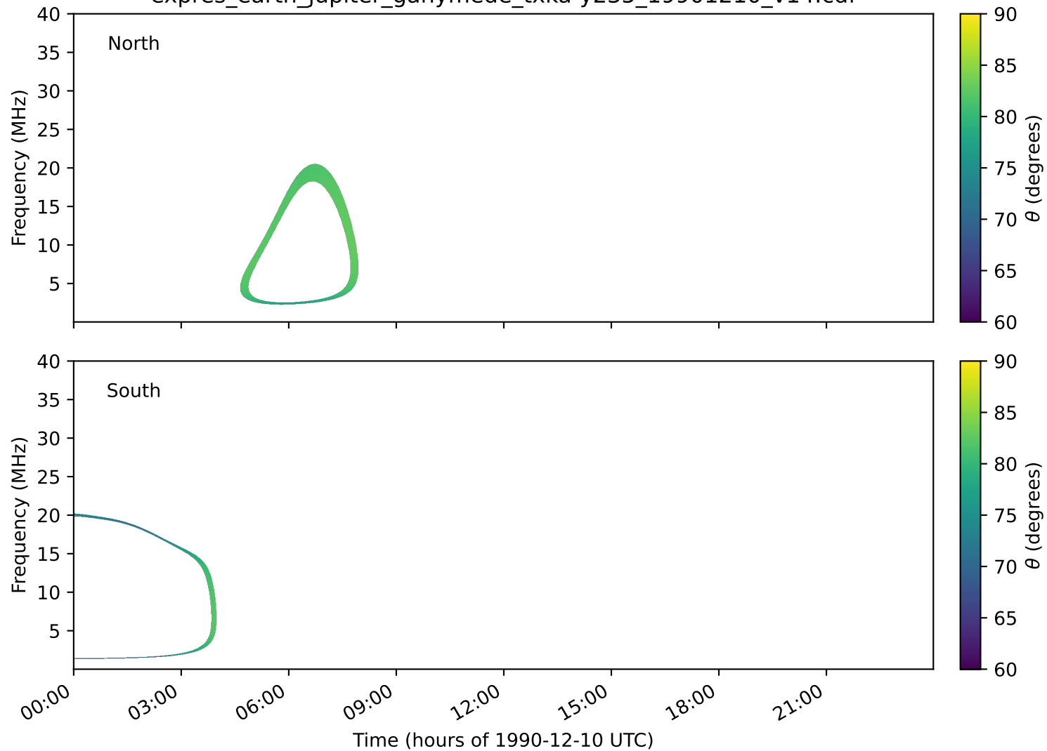
expres_earth_jupiter_ganymede_txka-y235_19901210_v14.cdf
