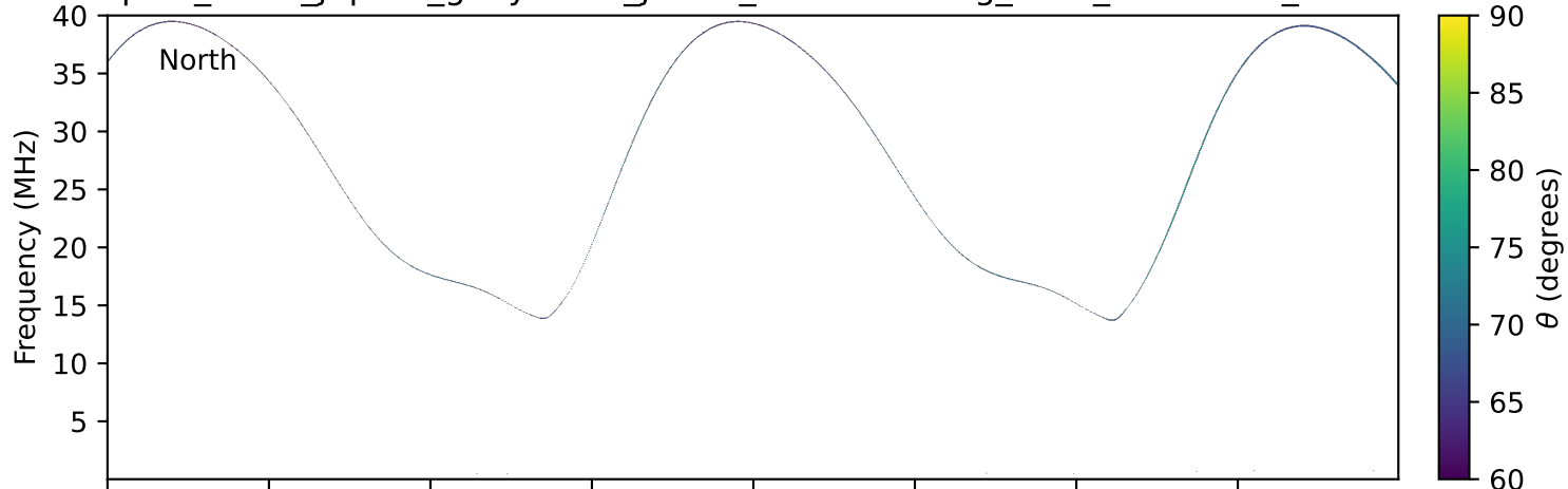
expres_earth_jupiter_ganymede_jrm09_lossc-wid1deg_3kev_19901230_v11.cdf
