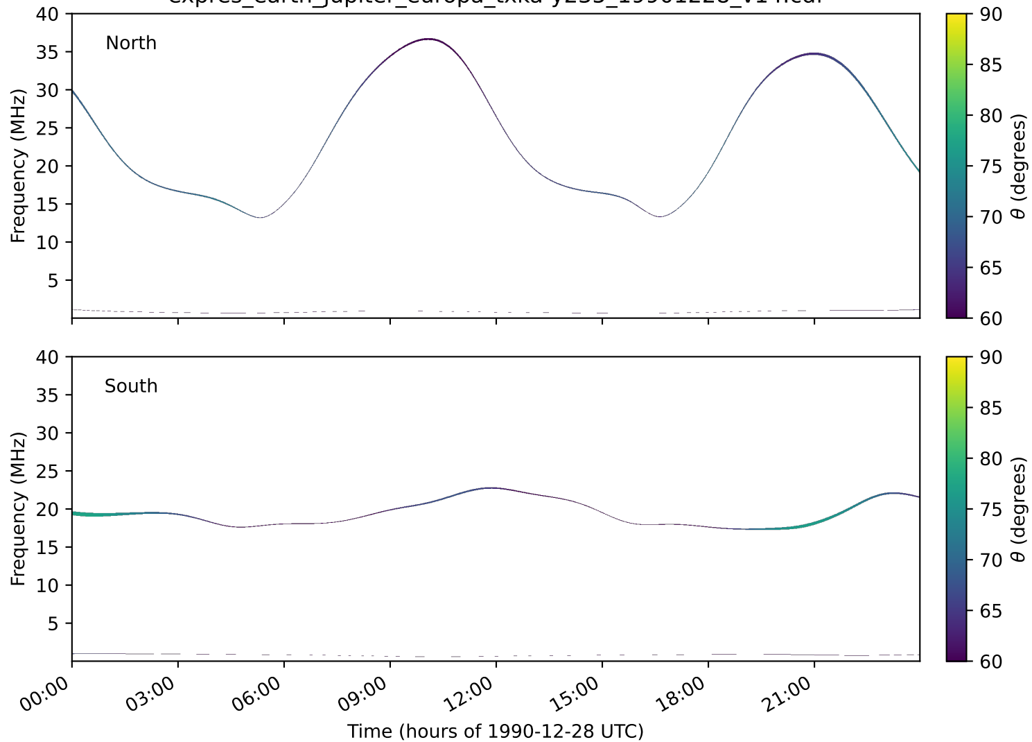
expres_earth_jupiter_europa_txka-y235_19901228_v14.cdf
