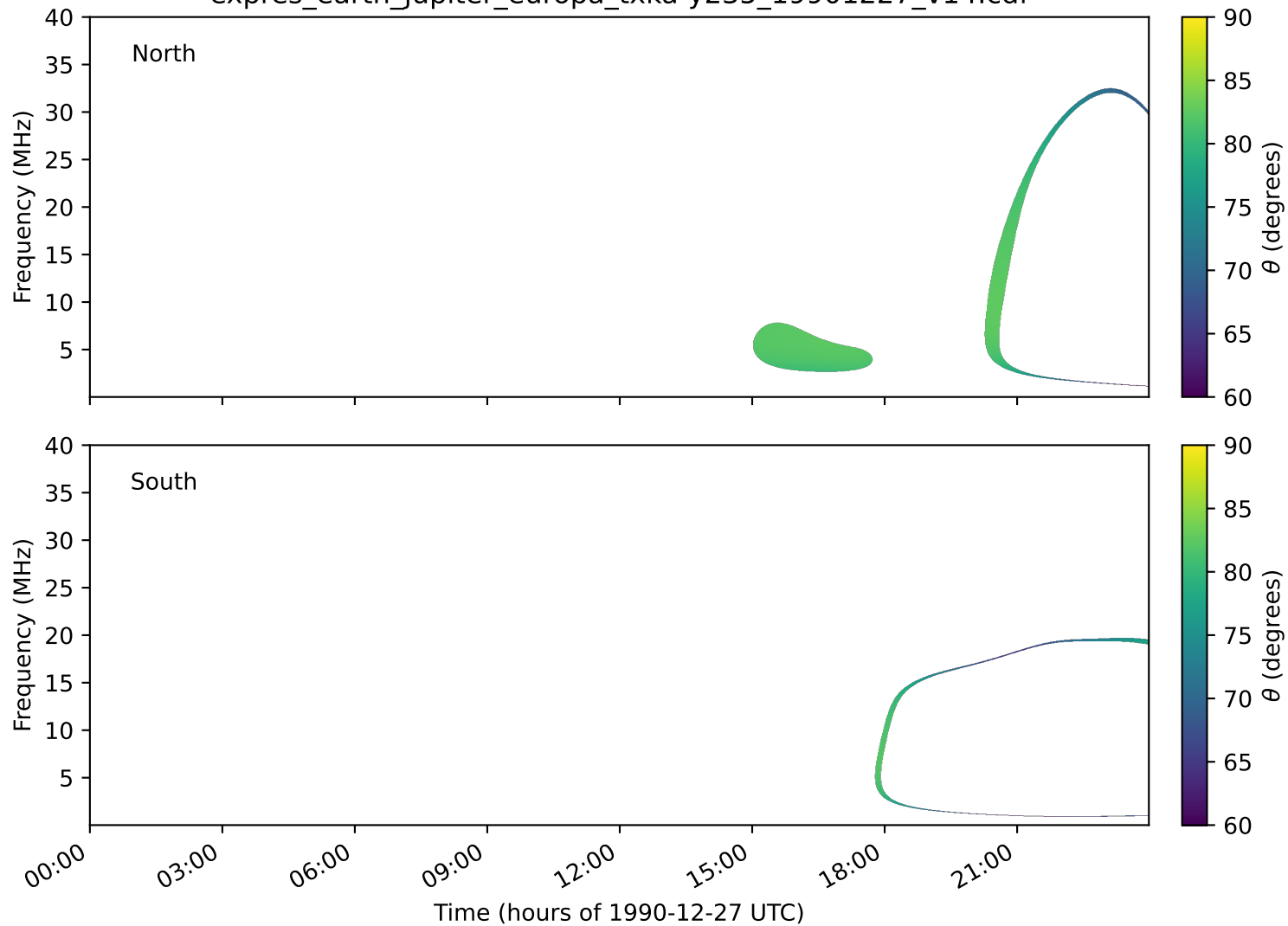
expres_earth_jupiter_europa_txka-y235_19901227_v14.cdf
