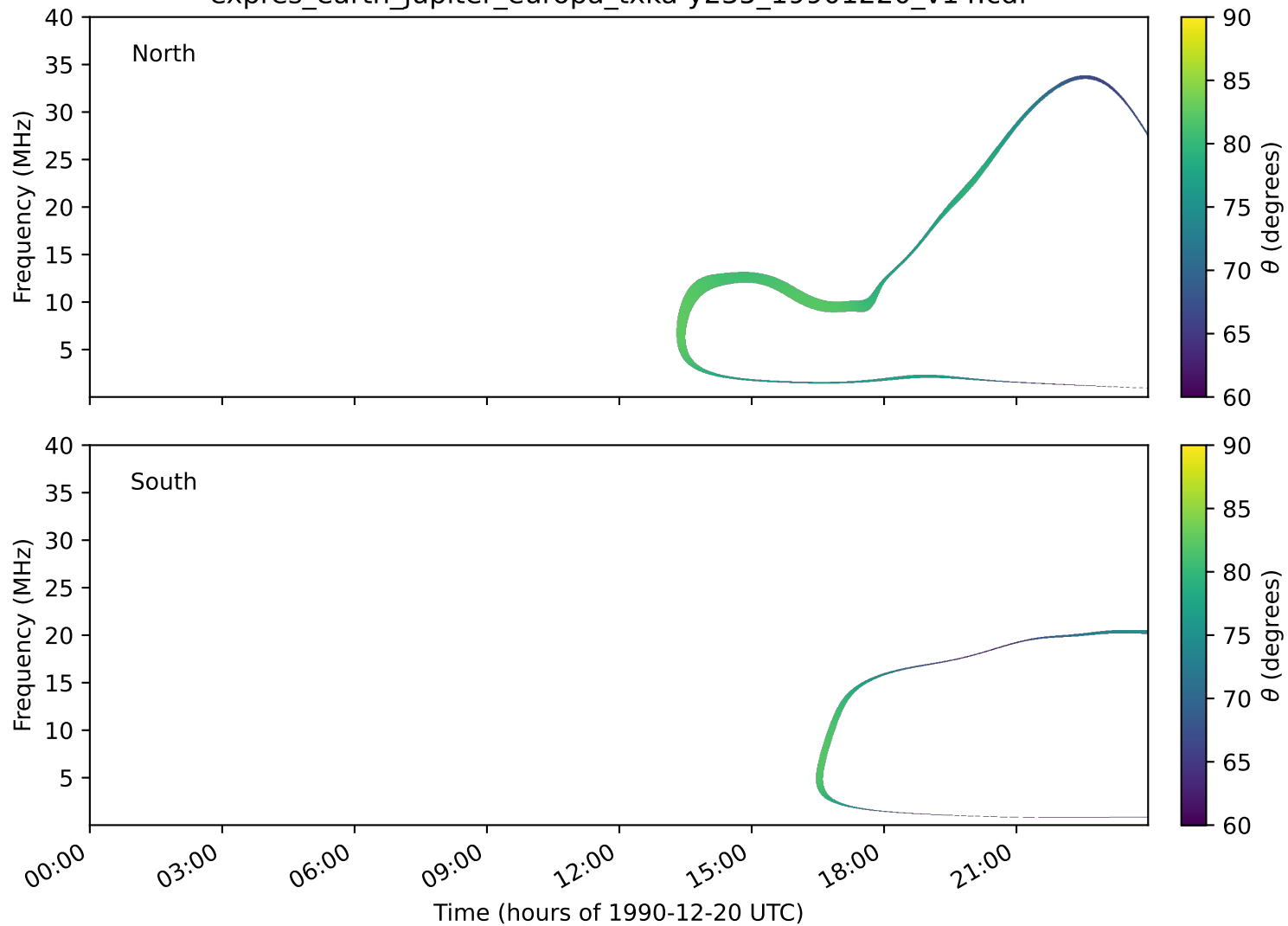
expres_earth_jupiter_europa_txka-y235_19901220_v14.cdf
