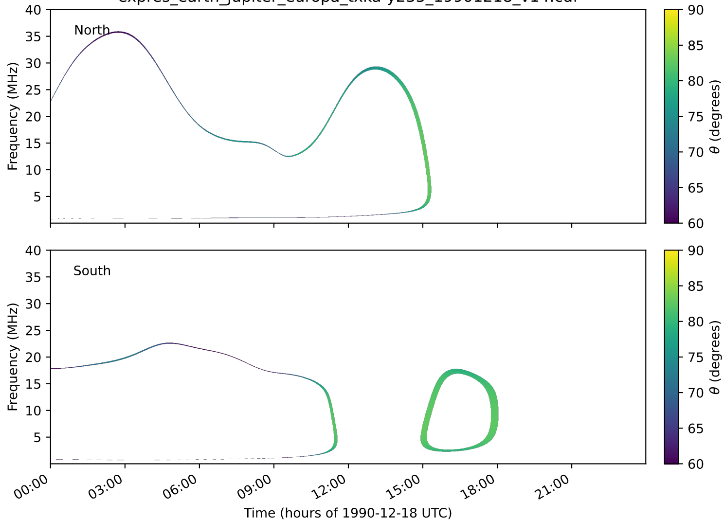
expres_earth_jupiter_europa_txka-y235_19901218_v14.cdf
