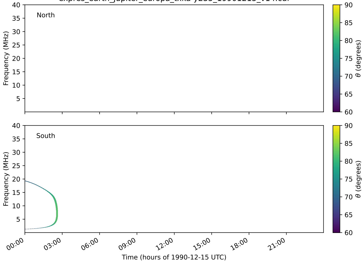
expres_earth_jupiter_europa_txka-y235_19901215_v14.cdf
