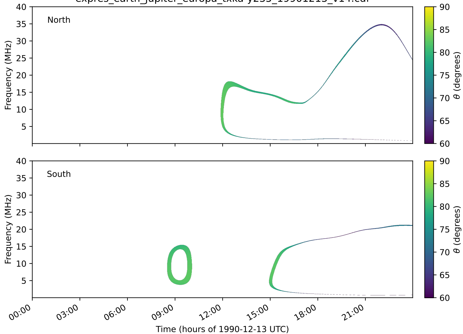
expres_earth_jupiter_europa_txka-y235_19901213_v14.cdf
