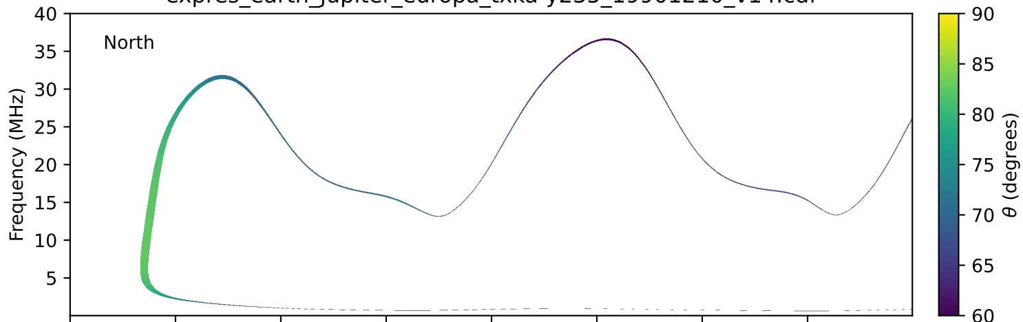
expres_earth_jupiter_europa_txka-y235_19901210_v14.cdf
