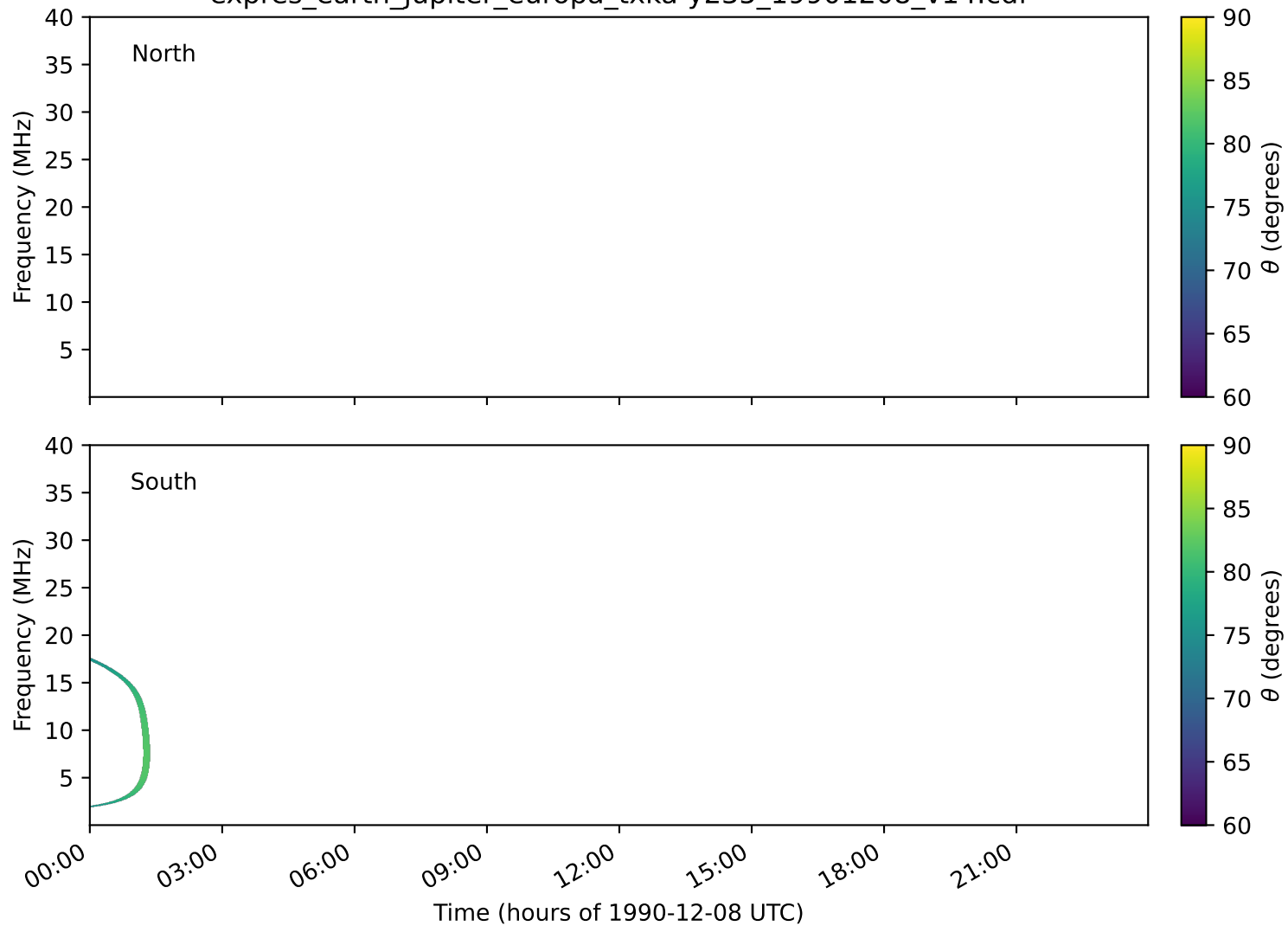
expres_earth_jupiter_europa_txka-y235_19901208_v14.cdf
