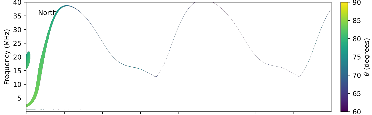
expres_earth_jupiter_europa_jrm09_lossc-wid1deg_3kev_19901203_v11.cdf
