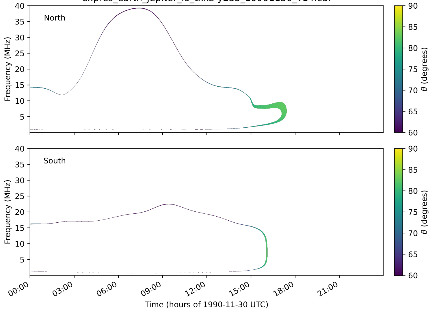
expres_earth_jupiter_io_txka-y235_19901130_v14.cdf
