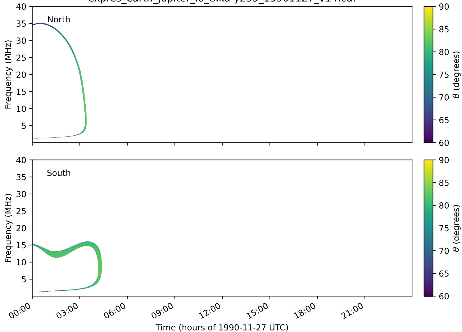
expres_earth_jupiter_io_txka-y235_19901127_v14.cdf
